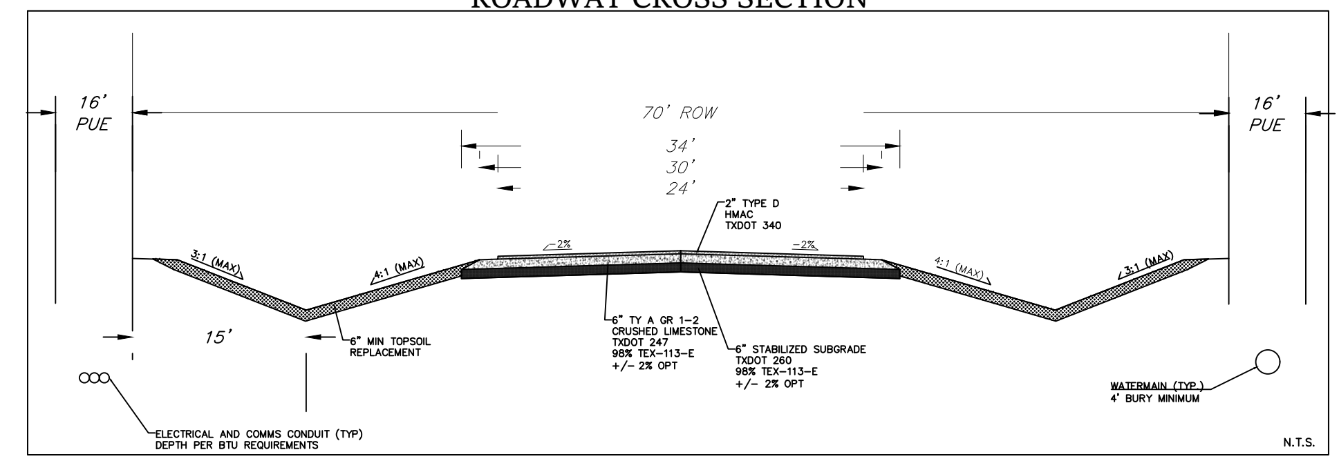
ROADWAY CROSS SECTION
